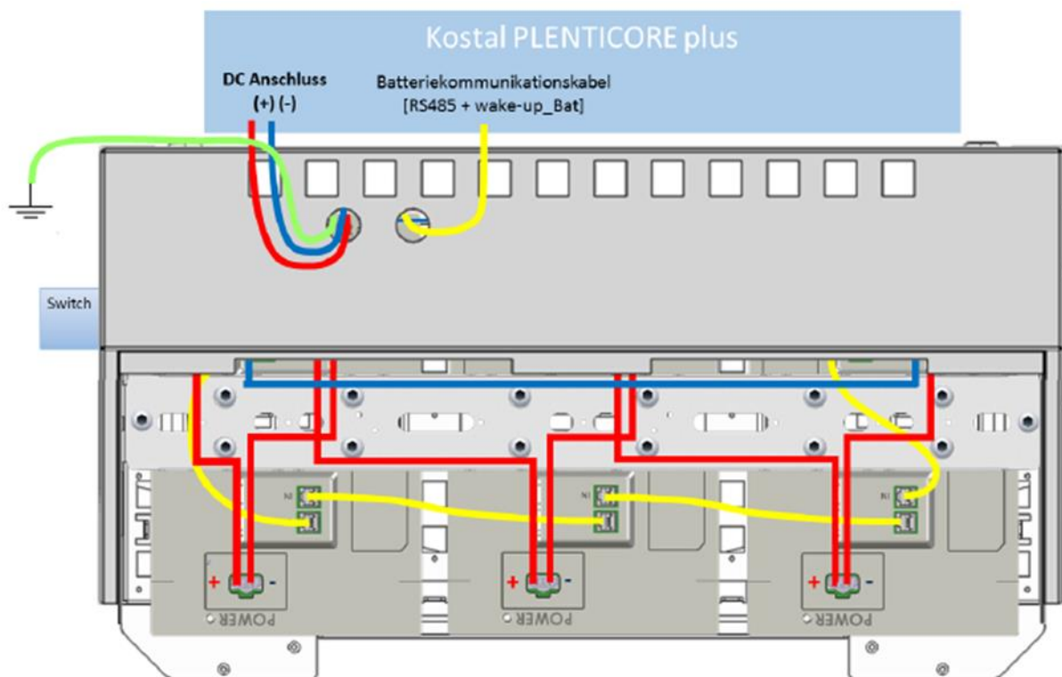
Figure 6: Connecting the PLENTICORE to the AXIstorage Li SH
