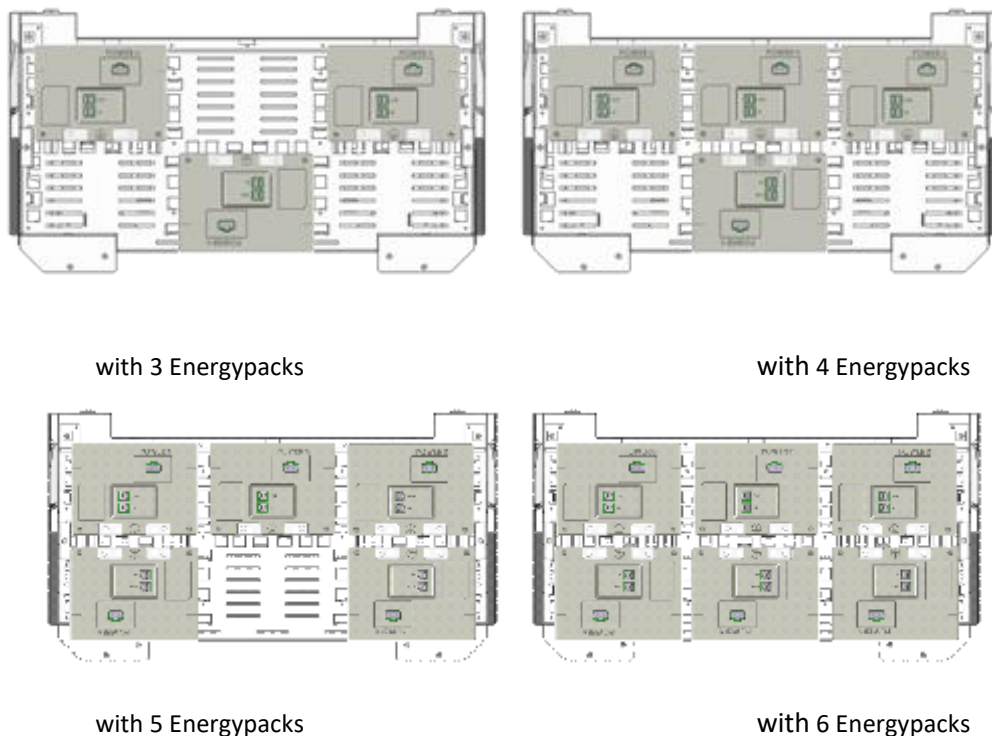
Figure 2: Insert 3 to 6 Energypacks
