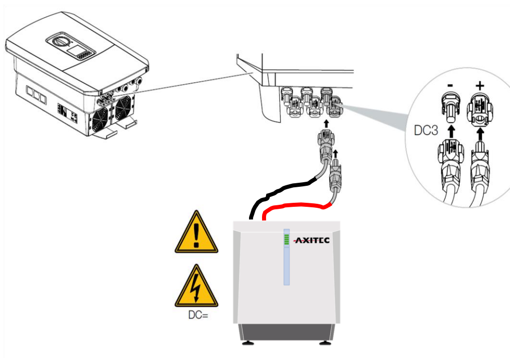
Figure 8: Connection of the PLENTICORE plus/BI - DC connection
