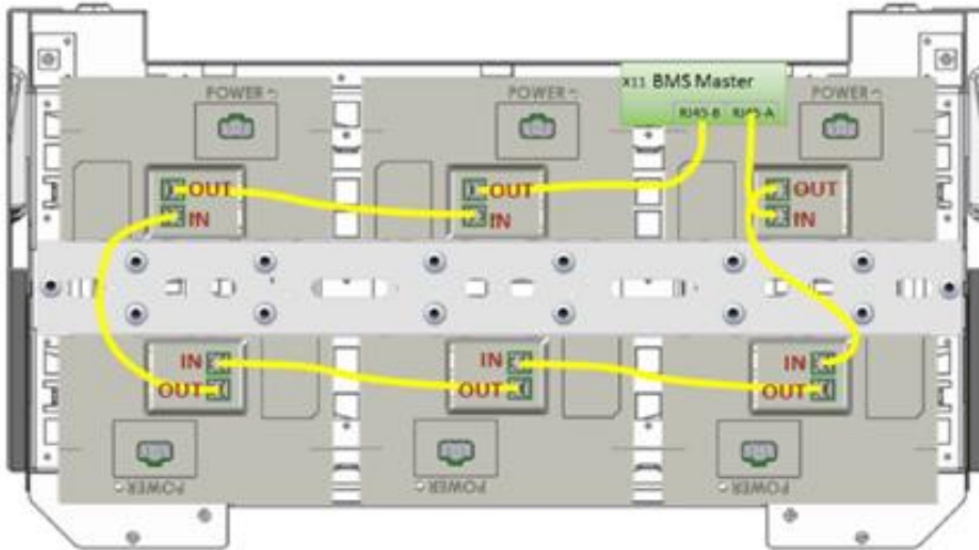
Figure 4: Connect the Energypack to the BMS master using the patch cables
