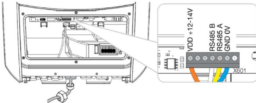
Figure 7: Connection of the PLENTICORE plus/BI - communication cable
