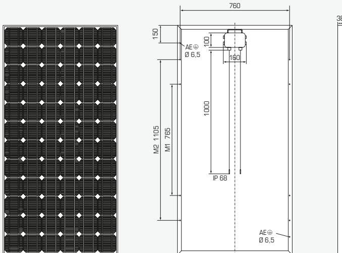
Alle Maße in mm/All dimensions in mm
