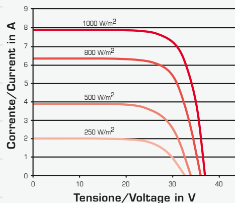
Esempio per/Example for AC-218P/156-60S
